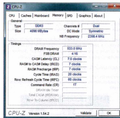
Program CPU-Z
